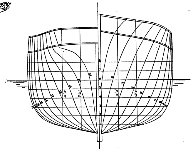
BODY PLAN
