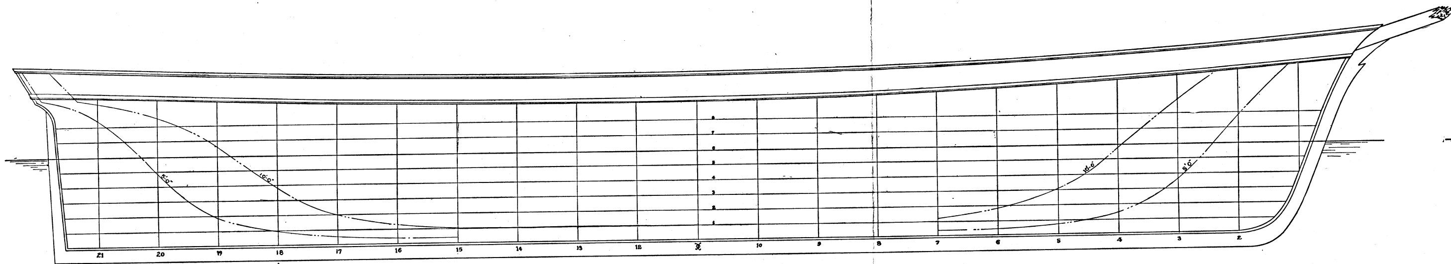
SHEER PLAN
