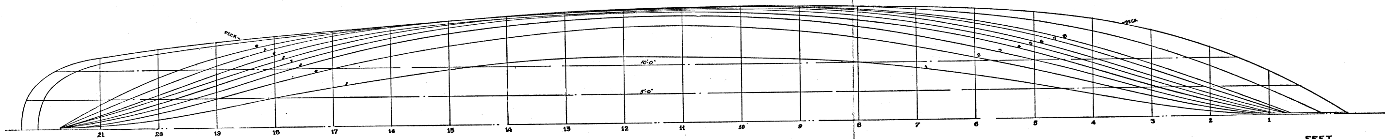
LINES
